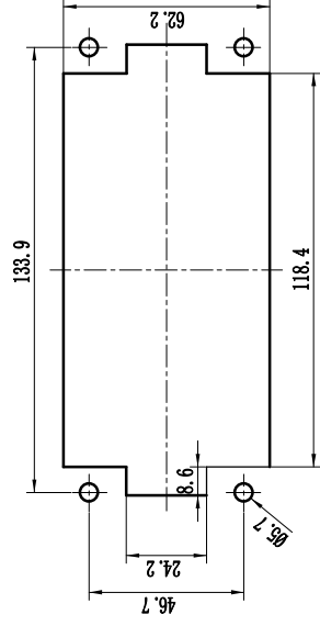
面板安装开孔图 Panel cut out
