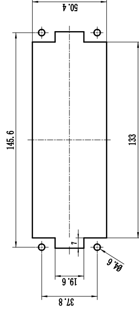
面板安装开孔图 Panel cut out
